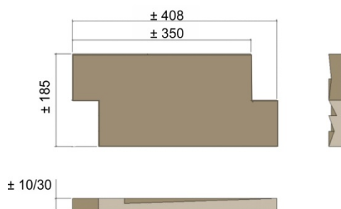
Thickness \pm 10/30 mm Piece internal Dimensions - Flat Elements
